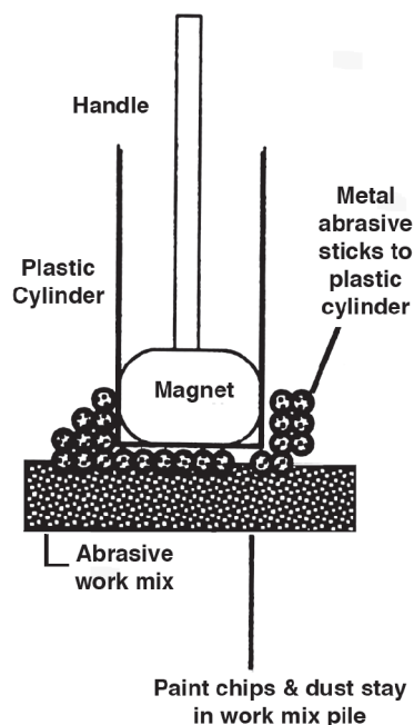
Figure 1 Separating Metallic Abrasive from the Work Mix Using a Sheathed Magnet
