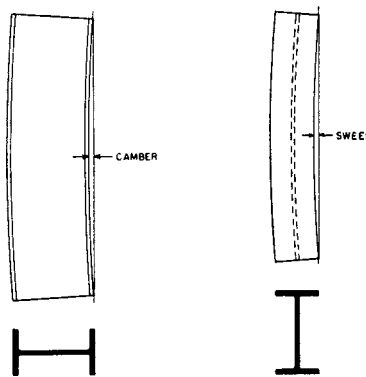
Positions for Measuring Camber and Sweep of W and HP Shapes
